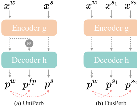
Figure 3. The two sub-frameworks, i.e. , UniPerb and DusPerb, that are integrated into our final UniMatch framework. The FP denotes feature perturbation, which is a simple Dropout in this work.
